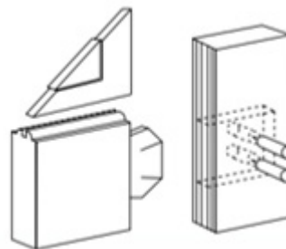
Dowelled construction
